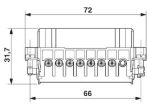
Female insert
