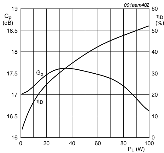
Fig 4. GSM EDGE power gain and drain efficiency as function of load power; typical values
