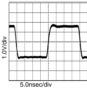
Fig.55 24.6MHz output waveform VDD=3.3V, at CL=15pF
