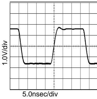
Fig.49 27MHz output waveform VDD=3.3V, at CL=25pF
