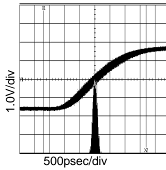
Fig.56 24.6MHz Period-Jitter VDD=3.3V, at CL=15pF
