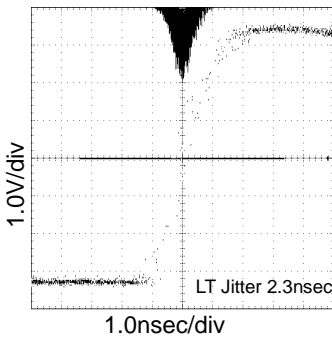
Fig61. 24.6MHz LT Jitter VDD=3.3V, at CL=15pF
