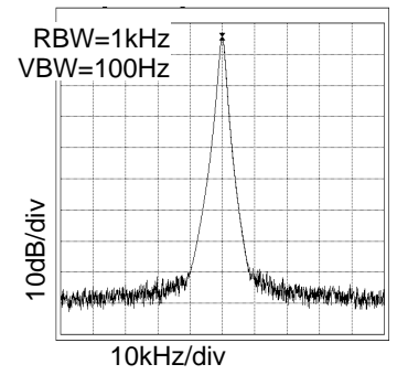
Fig.57 24.6MHz Spectrum VDD=3.3V, at CL=15pF
