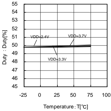
Fig.111 16.9MHz Temperature-Duty
