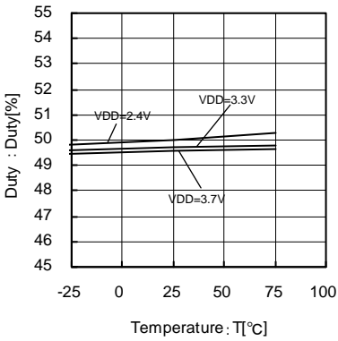
Fig.102 36.9MHz Temperature-Duty
