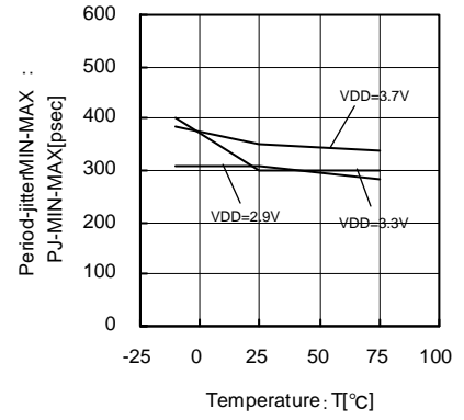
Fig.41 18.4MHz Temperature-Period-Jitter MIN-MAX
