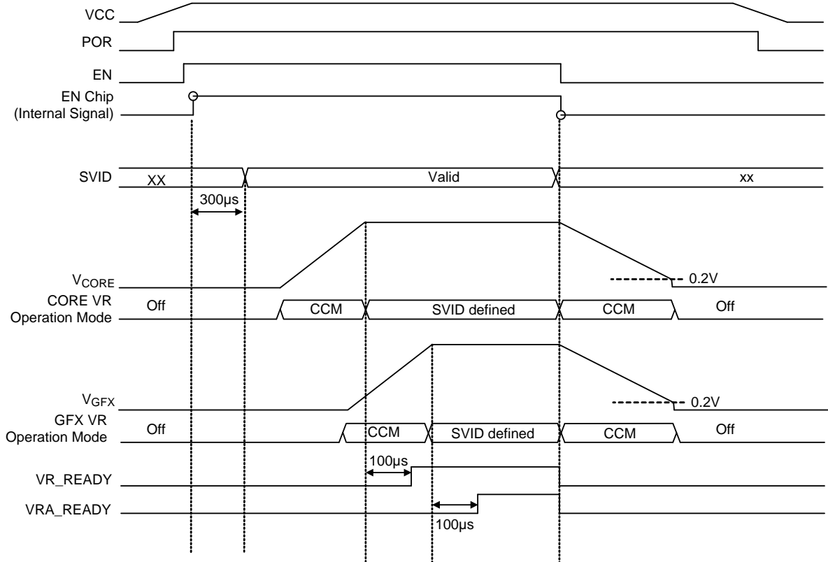
Figure 7 (a). Power sequence for RT8168B ( V_{INL\_CORE} = V_{INL\_GFX} = 0V )
