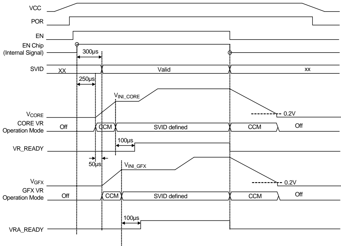
Figure 7 (b). Power sequence for RT8168B ( V_{INL\_CORE} \neq 0, V_{INL\_GFX} \neq 0V )
