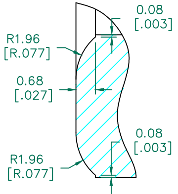
DETAIL "A" CHAMFER SCALE=8:1
