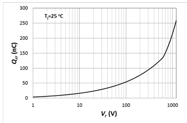
Recovery Charge
