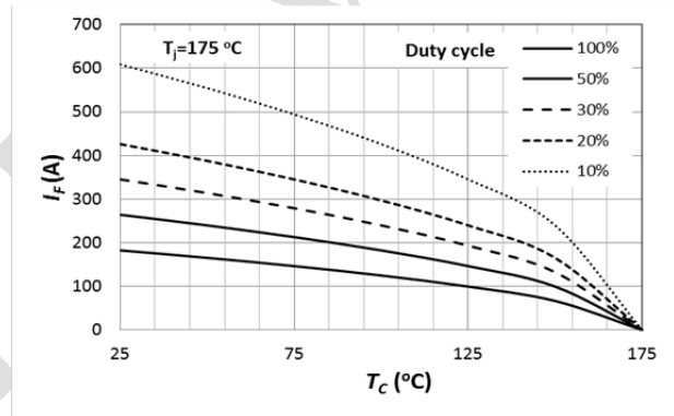
Current Derating
