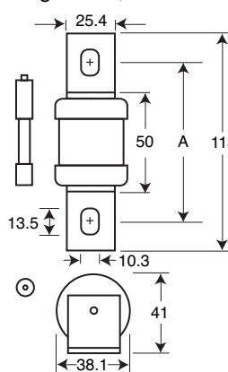
Figs. 4 & 5 "A" Dimensions
