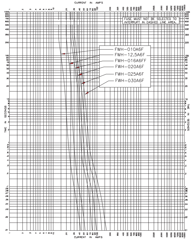
Time-Current Curve
