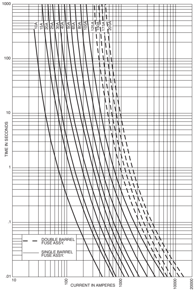
Time-Current Characteristics – Total Clear
