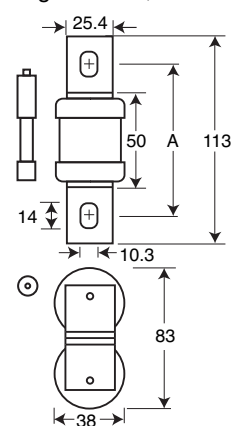
Figs. 4 & 5 "A" Dimensions
