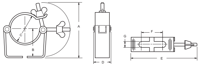
9078A67G04 3" Diameter Clip
