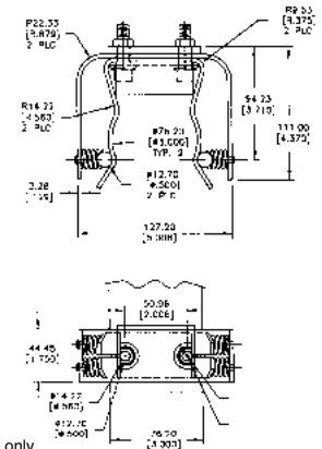
9078A67G04 3" Diameter Clip
