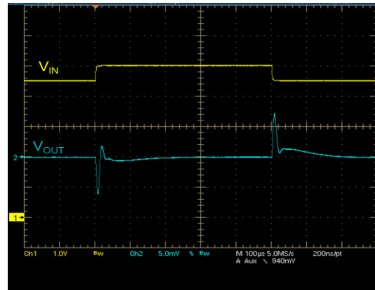
Figure 13: Line transient ( I_{OUT} = 1\text{ mA} )
