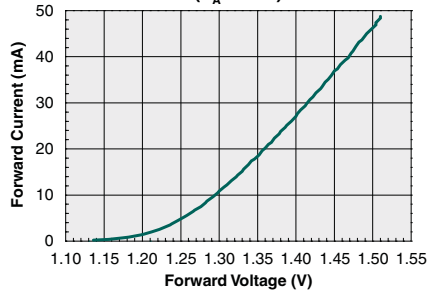
Typical LED Forward Voltage vs. Forward Current (T A =25°C)
