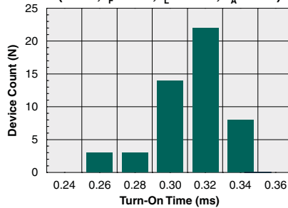
Typical Turn-On Time (N=50, I F =5mA, I L =60mA, T A =25°C)
