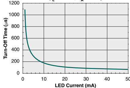
Typical Turn-Off Time vs. LED Forward Current (I L =60mA, T A =25°C)
