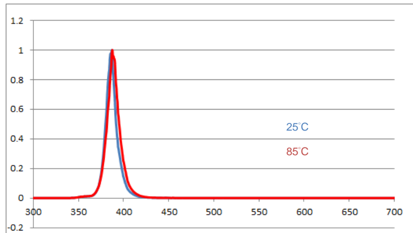
Fig 2. Relative Spectral Distribution at T j = 25°C & 85°C
